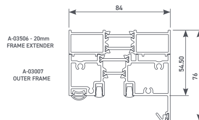
Standard outer frame with 20mm extender
